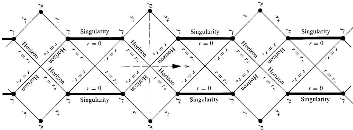
Figure 54: This figure shows the conformal diagram of Reissner-Nordström spacetime. Hypercomplex coordinates on chronos and chiros are well suited to defining a continuous parameter through the periodic boundaries. Where we have previously made reference to the Kerr–Newman metric of a charged rotating black hole, the Reissner–Nordström metric describes a a charged black hole with no net angular momentum.
