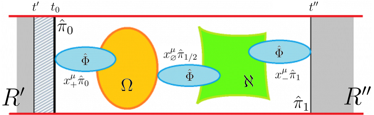
Figure 9: This figure illustrates the region of figure 7 between t_0 and t'' . If one considers the third \hat{\pi} component in the middle as x_\emptyset^\mu \hat{\pi} then it is very easy to see where the (\Phi\pi)^3 term comes from in \alpha_{MCM} . Simply let the non-unitary component be such that each \hat{\pi} is inflated by \Phi from one moment to the next. In a sense we can say \hat{\pi}_{1/2} is out of phase with the other two \hat{\pi} 's (the normal sense of \pi/2 orthogonality) and it is \hat{\pi}_0 and \hat{\pi}_1 that give, speculatively at least, the 2\pi for \alpha_{MCM} = 2\pi + (\Phi\pi)^3 .
