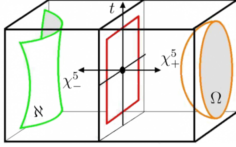
Figure 32: The original graphical iteration of the MCM unit cell is, perhaps, the most intuitive representation of its important geometric features.
