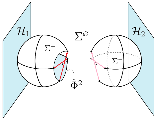
Figure 86: In this book we have focused on attaching the small sphere to the circle to achieve SU(2) \otimes U(1) but for the complete standard model we need to achieve SU(3) \otimes SU(2) \otimes U(1) which is the plane with a 2-sphere attached on one side and a 3-sphere on the other. This figure does not directly motivate the group theoretical structure of the standard model but it does demonstrate an intuitive arrangement for the j \rightarrow j + 2 change in the level of \aleph under \hat{M}^3 . If both \mathcal{H}_1 and \mathcal{H}_2 have a sphere with two \hat{\Phi} objects on the right side, then on the left side of \mathcal{H}_2 we could, for instance, have a sphere missing the \hat{\Phi}^2 which it receives from \mathcal{H}_1 during propagation across the unit cell with the inversion operation on the Riemann sphere. This figure shows a double inversion where the first inversion moves the sphere's origin to p \in \Sigma^\emptyset and the second moves it to a point in \mathcal{H}_2 .
