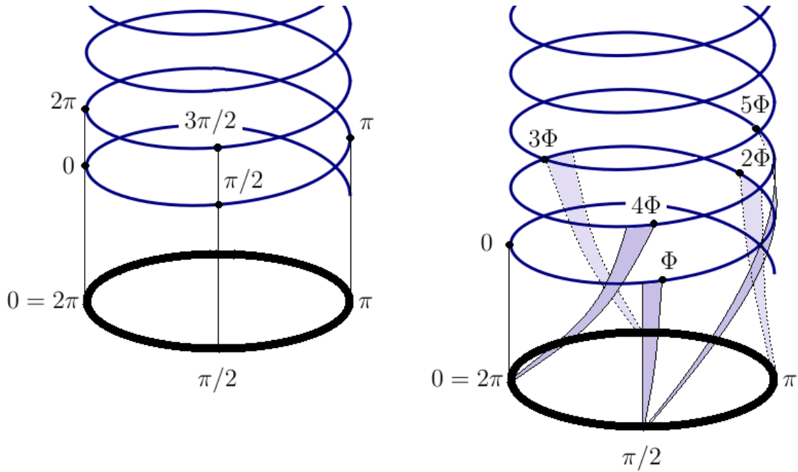
Figure 78: Here we can see an intuitive placement for the idea to encode half of a \text{co-}\hat{\pi} ( \pi/2 \approx 1.57 ) on each \hat{\Phi} (because \Phi \approx 1.62 .) Each purple region has an element \Delta = \Phi - \pi/2 that can be associated with \Sigma^\varnothing in the base space. We will establish complex behavior when we make a representation where the \Sigma^\varnothing element has non-zero width. The affine parameter along the helix that contains the covering space is a natural object for such a definition.
