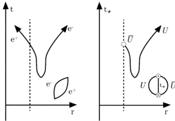
Figure 10: This is the the mechanism from reference [7] through which we claimed to have unified gravity and electromagnetism, and here we point out that reference would have been better titled Dark Energy in the Modified Cosmological Model with Ancillary Takeaways . We use the “in” \odot and “out” \otimes diagrammatic notation of EM to show the places where the piecewise bulk geodesics are joined across different tiers of infinitude (levels of \aleph ) in {}^*\mathbb{C} . The original caption for the diagram was, “The Feynman diagrams of gauge theory generate surfaces which represent interacting strings [16]. On the left: electromagnetic pair creation near the horizon. On the right: polarized gravitational pair creation.” This figure is adapted from reference [17] and it went unfortunately uncited when we used it in reference [7].
