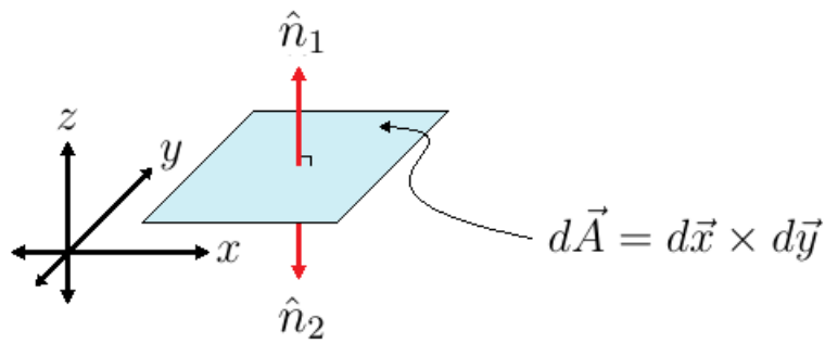
Figure 82: This figure demonstrates a symplectic 2-form. Noting that the 1/2 factors in equation (4.165) come from the double counting in the Einstein notation we see that when \hat{n} is a unit vector |\hat{n}|=1 the possible values for dS = d\vec{A} \cdot \hat{n} are \pm dx dy depending on which normal vector is used.
