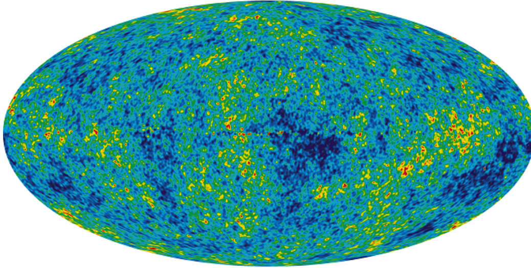
Figure 48: The results of the WMAP experiment show that the angular scale of temperature fluctuations in the cosmic microwave background is about 1^\circ implying that the spacetime on the interior of the CMB has very little or no net curvature.
