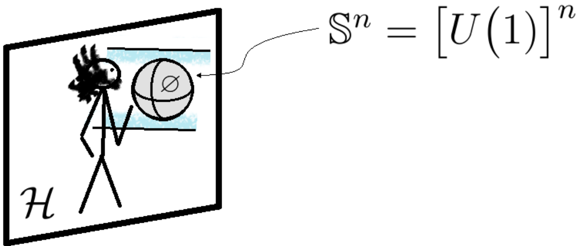
Figure 43: This figure calls attention to the psychological nature of physics. This figure calls further attention to the application of the sphere theorem to the framework depicted in figures 37-42.
