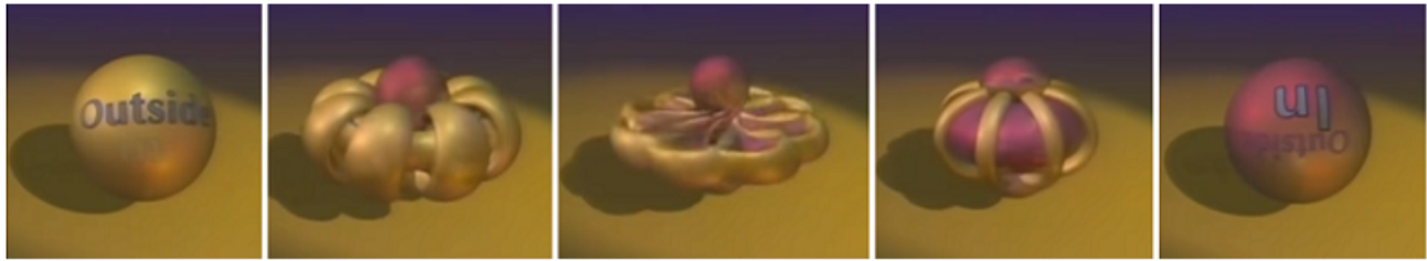
Figure 81: The sphere theorem offers another method to invert the Riemann sphere beyond the ordinary discrete inversion map \zeta = 1/\xi . In addition to swapping the interior and exterior regions, this inversion operation also turns the sphere upside down which will implement the changing anchor points in the associated vector field. The normal vector pointing outward from the north pole of the sphere in the first frame becomes an inward pointing normal vector anchored to the south pole in the last frame. The sphere theorem demonstrates an important application in which we must consider the differential element of surface area as dS_i = \pm \epsilon_{ijk} dx^j dx^k instead of simply dS_i = \epsilon_{ijk} dx^j dx^k . This figure is taken from reference [65]
