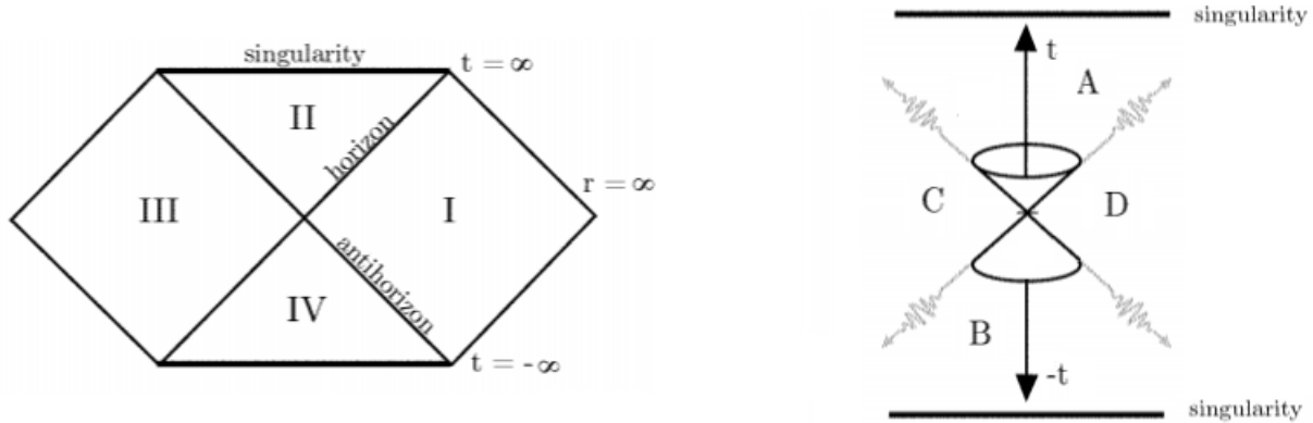
Figure 46: On the left is the Penrose diagram of a Schwarzschild black hole. On the right is a quasi-Minkowski diagram describing the big bang. It shows two future light cones opening in opposite directions away from the big bang. The arrows on the right indicate the arrows of time in the universes U and \bar{U} .
