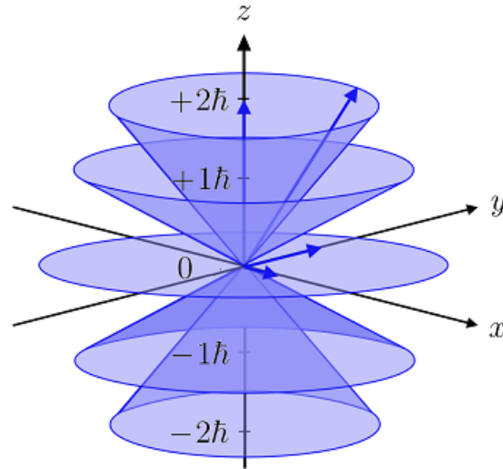
Figure 60: This figure shows the possible angular momentum configuration for l=2 . For any l -state there are 2l + 1 possible values of m giving the 2 \times 2 + 1 = 5 possible values shown in this figure which is mostly taken from Wikipedia.
