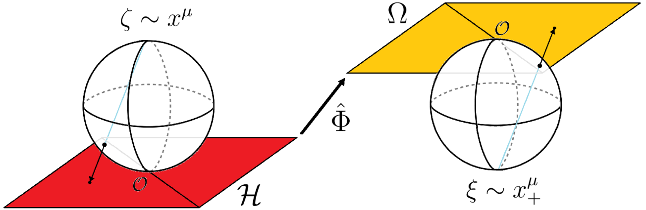
Figure 6: This figure shows the bijection between a sphere and two planes: two flat slices of some bulk. \mathcal{O} marks the origin of coordinates on each chart. This figure differs from figure 4 because here the sphere connects \mathcal{H} to \Omega but in figure 4 \hat{\Phi} connects \mathcal{H}_1 to \mathcal{H}_2 . Where figure 4 shows what we called the 5D p , the point \mathcal{O} on the right of this figure would be the first 4D p . Since the Gel'fand triple is constructed by first taking a subspace of \mathcal{H} this figure suggests that we should examine a possible reversal of the association of \aleph' and \Omega' with dS and AdS ( \aleph and \Omega .)
