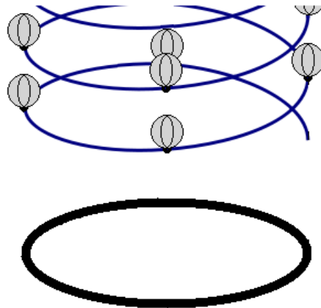
Figure 79: By compactifying the extra elements \Phi - \pi/2 it is possible to recover the trivially projective covering space. This figure is evocative of the mechanism through which points in spacetime become the Riemann sphere in twistor space.
