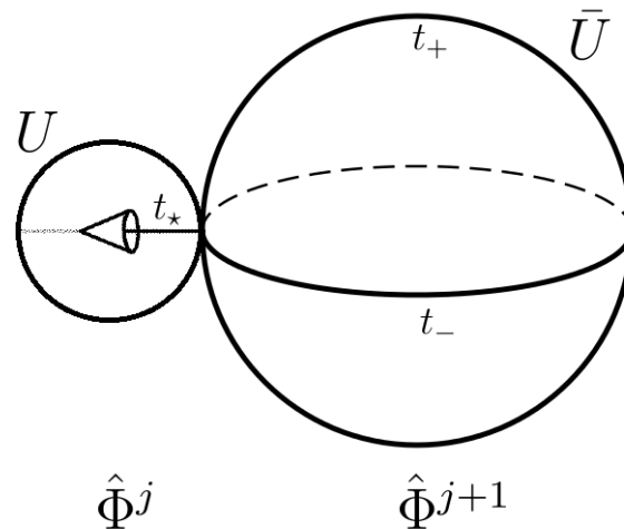
Figure 50: This figure shows a universe U which will experience dark energy due to the gravitational pull of \bar{U} on a higher level of \aleph . If we convert to the t_{\pm} representation in U then we could add another universe on \hat{\Phi}^{j-1} which would experience dark energy in its t_* representation due to the pull of U .
