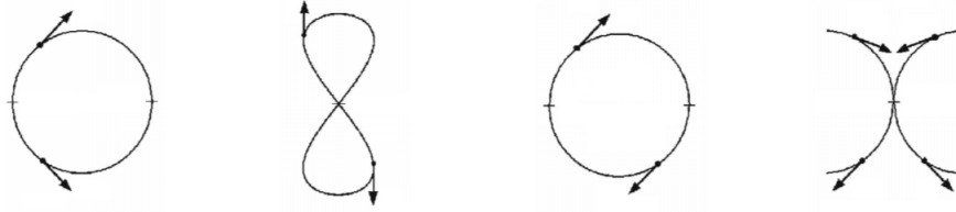
Figure 22: If the figure on the left represents a condition of symmetry then the output of the operation to the right will represent a condition of antisymmetry. Bosons have symmetric wavefunctions and fermions have antisymmetric wavefunctions.
