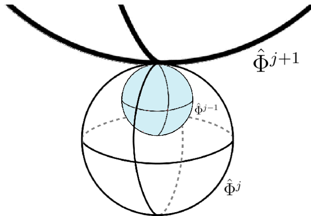
Figure 39: When repeated many times, the operations in figure 38 can generate the nested fractal structure developed in reference [8] to argue against the Riemann hypothesis. The three spheres in this figure are on different levels of \aleph which means that the radius of each larger sphere is infinite with respect to the radii of the spheres nested within.
