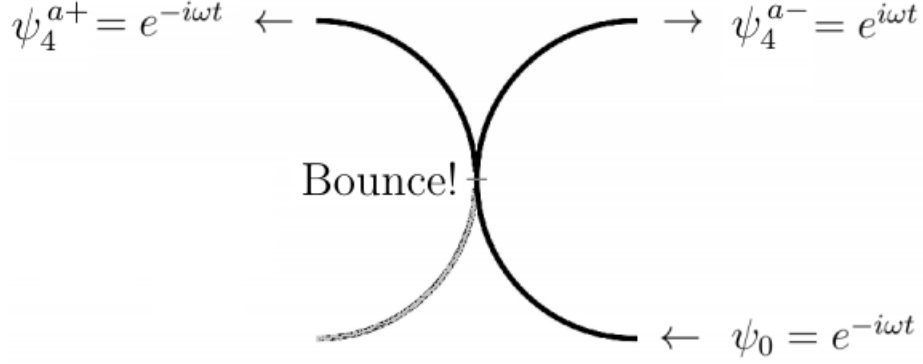
Figure 31: A plane wave incident on the bounce state from the bottom right. The bounce is generally understood by now to lie at either the endpoints of the MCM unit cell or the central point corresponding to p \in \Sigma^\emptyset . In incident wave can be either transmitted or reflected by the bounce.
