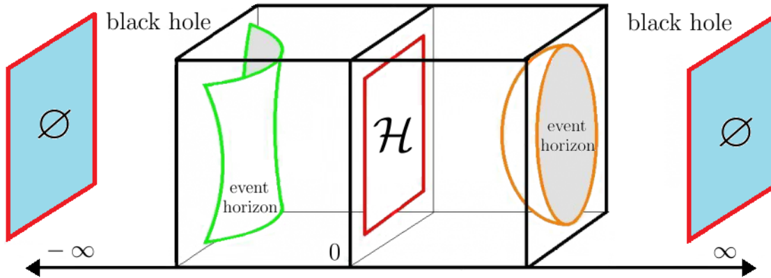
Figure 55: When we join across levels of \aleph with singular topology \emptyset we can say that the region denned by \aleph and \Omega is surrounded by black holes (pictured) or equivalently \mathcal{H} can be the singularity denned within the \{\aleph, \Omega\} event horizons. In the latter case we directly obtain the notion of a universe inside a black hole.
