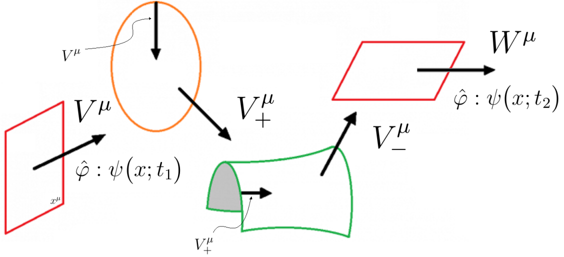
Figure 18: The new object \hat{\varphi} encodes the quantum sector in the MCM unit cell along side the ontological basis \{\hat{i}, \hat{\Phi}, \hat{2}, \hat{\pi}\} which are used, among other things, as a non-coordinate basis for general relativity. This system needs to be able to support at least two distinct phases: decoherence and stability. The non-decoherence mode of repeated measurement is such that all the V are linearly dependent on \hat{\Phi} . Then Q = |V^\mu - W^\mu| = |\hat{\Phi} - \hat{\Phi}| = 0 .
