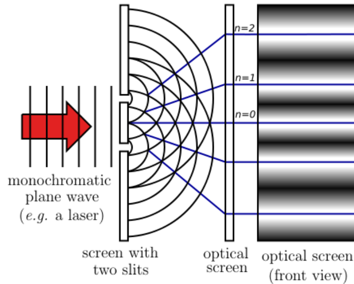
Figure 88: Wave interference requires that the flux incident on the diffraction screen pass through both slits equally. This figure is taken from Wikipedia and ignores the decreasing amplitudes of the maxima away from the beamline.
