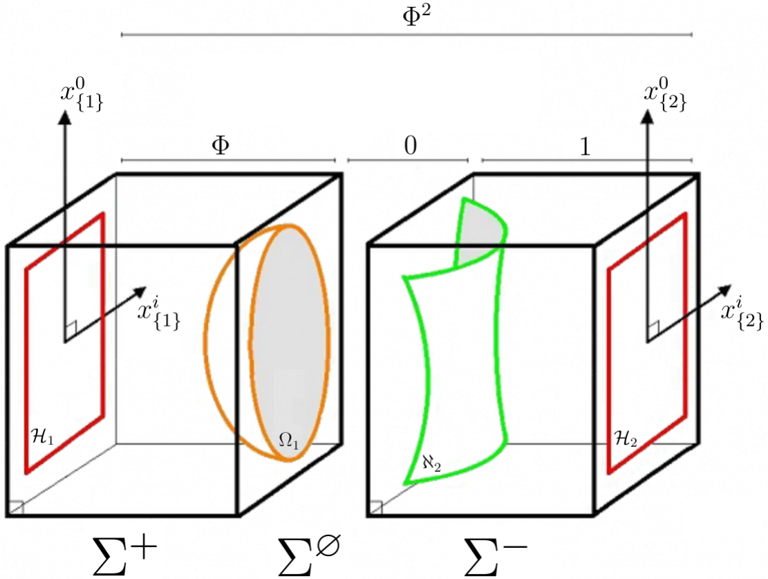
Figure 1: The region between two adjacent moments of psychological time: \mathcal{H}_1 and \mathcal{H}_2 . The arrangement immediately suggests a gravitational pilot wave formulation as the path to evolve through the discontinuity of the as-yet-undescribed region inside the null interval between \Omega_1 and \aleph_2 but we will introduce another simpler formulation in this book. We will introduce new \chi_{\emptyset}^A coordinates to accommodate this representation wherein x^\mu \in \mathcal{H} are moved away from the center of the MCM unit cell where we have depicted them in previous work. \chi^5 is the horizontal direction across this figure. This figure uses the values \Phi^2 , \Phi , and 1 to demonstrate \Sigma^\emptyset but there are many such arrangements.
