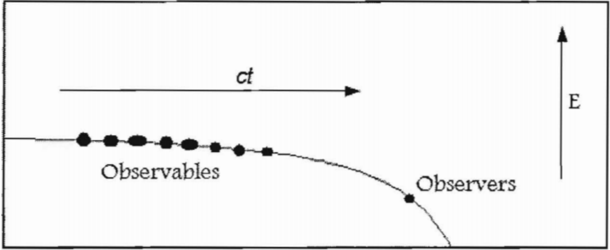
Figure 5: This figure seeks to demonstrate how dark energy is a solution to the Poisson equation inside the cosmological unit cell.
