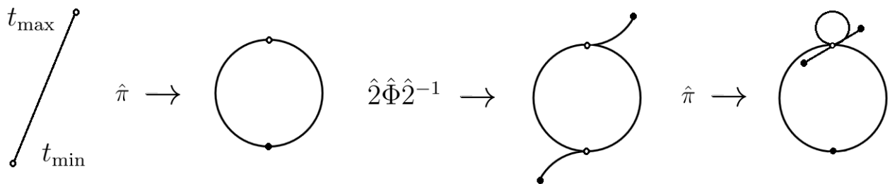
Figure 42: When we take the operator \hat{2}\hat{\Phi}\hat{2}^{-1} such that \hat{\Phi}^j \rightarrow \hat{\Phi}^{j+1} then there is an intuitive association that \hat{2} takes a qubit out of \mathcal{H}_1 at which point \hat{\Phi} operates before we use \hat{2}^{-1} to put the qubit back into \mathcal{H} at \mathcal{H}_2 .
