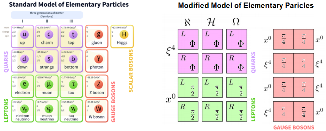
Figure 28: The 4 \times 4 symmetry of the standard model is broken by the spin-0 H scalar boson but the 4 \times 4 symmetry of the modified model is completed with the spin-1 G and \zeta gauge bosons. Notice how the labeling, up to an extra \Phi in each generation of matter particle, gives \alpha_{MCM} = (\Phi\pi)^3 + 2\pi . See reference [11] for details regarding the modified model of elementary particles.
