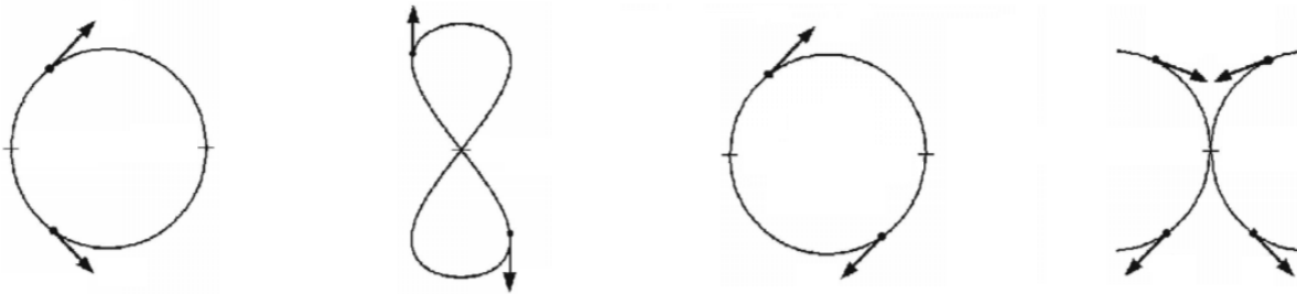
Figure 44: The MCM proposes to wrap the ct axis of the Minkowski diagram around a cylinder.
