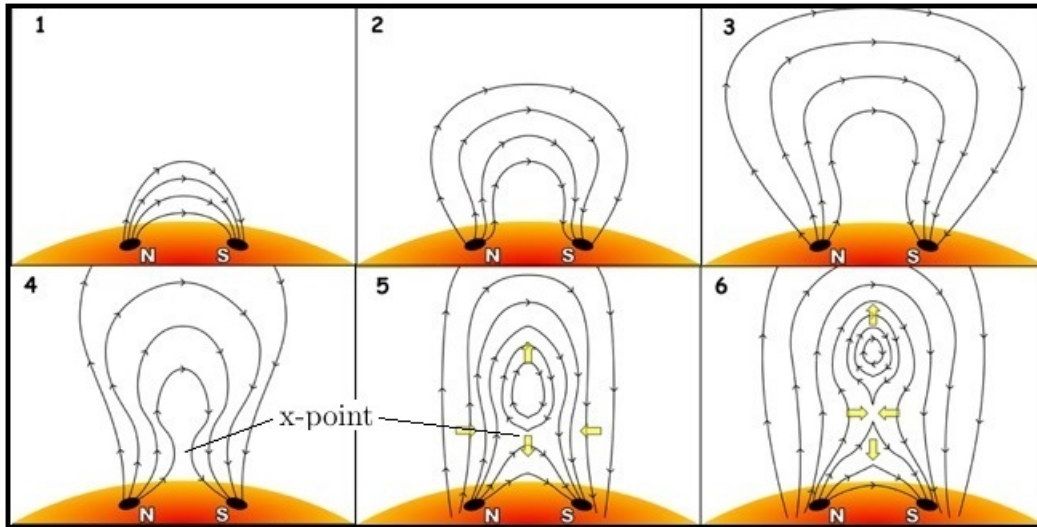
Figure 70: The angle of intersection of the field lines between panes four and five, the so called x-point, is not preserved throughout the field evolution so the evolution operator cannot be constructed from conformal transformation operators. This figure is adapted from one found on website of the Department of Astronomy of the University of Wisconsin.
