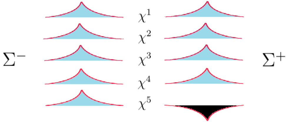
Figure 95: \chi^5 has an antisymmetric wavefunction because there is topological obstruction at \chi^5 = 0 that invokes a twisted path around infinity.
