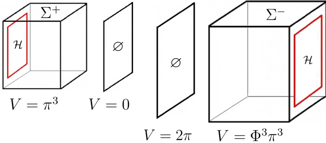
Figure 33: This figure shows the relative volumes of the major elements of the unit cell. Notably \emptyset must have A = \pi^2 on the left and A = \Phi^2\pi^2 on the right. Therefore during \hat{M}^3 \emptyset can be uniformly rarefied by \Phi or it can be rarefied only in one direction (probably the timelike direction) by \Phi^2 . However, we expect that the unit cell centered on \mathcal{H} will have the same area on both sides as in figure 34.
