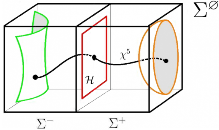
Figure 12: \mathcal{H} is not at the point p \in \Sigma^\emptyset . \Sigma^\emptyset lies all around the outside of this representation.
