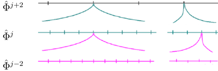
Figure 66: This figure shows tiers of infinitude as \{\hat{\Phi}^{j+2}, \hat{\Phi}^j, \hat{\Phi}^{j-2}\} . When this figure appeared in chapter one there was an intuitive idea that this should show three adjacent levels of \aleph but clearly it does not. This shows the entire infinite expanse of the central level being like a point in the upper level so it necessarily skips the intermediate level. A finite element on \hat{\Phi}^{j+1} is like a point on \hat{\Phi}^{j+2} or the entire real line on \hat{\Phi}^j .
