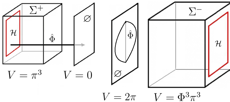
Figure 90: This figure shows where we can obtain \alpha_{MCM} = 2\pi + (\Phi\pi)^3 via manner of rarefaction demonstrated by figures 33 and 34. A rotation of the second \hat{\Phi} about the first \hat{\Phi} axis will directly implement the torsion so this is a very natural representation. It is evocative of figure 91.
