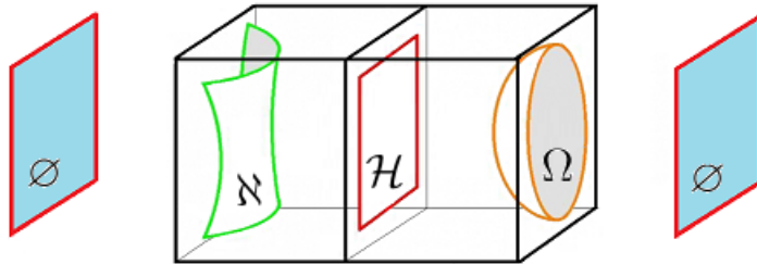
Figure 67: We have previously cited a problem with the physical interpretation for the extension of the MCM spin scheme to spin-2. The scheme in this figure which includes \emptyset assuages the interpretive problem so spin-2 fundamental MCM particles should not be ruled out on interpretive grounds alone.
