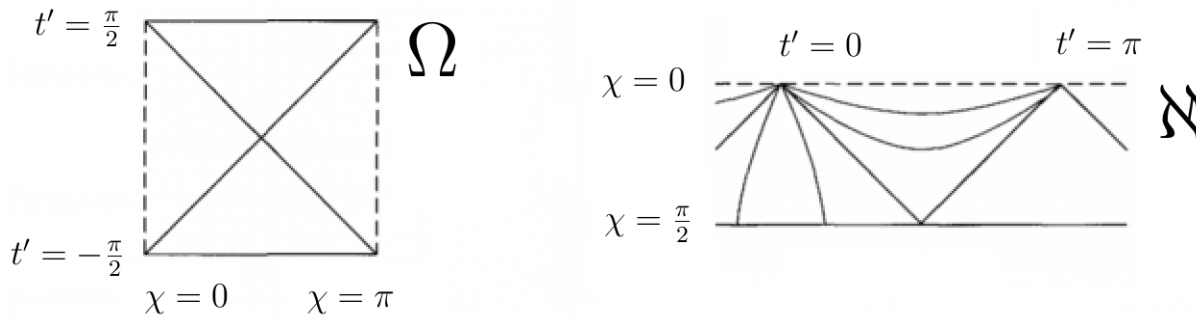
Figure 74: This figure contains conformal diagrams of de Sitter space and anti-de Sitter space.
