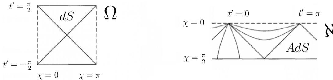
Figure 29: These conformal diagrams are most appreciatively reproduced from Carroll’s textbook, reference [17]: Spacetime and Geometry: An Introduction to General Relativity .
