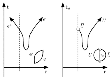
Figure 91: This figure from reference [7] (excerpted from reference [17]) demonstrates the general principle of \hat{\Phi} pointing to and lying within a worldsheet.
