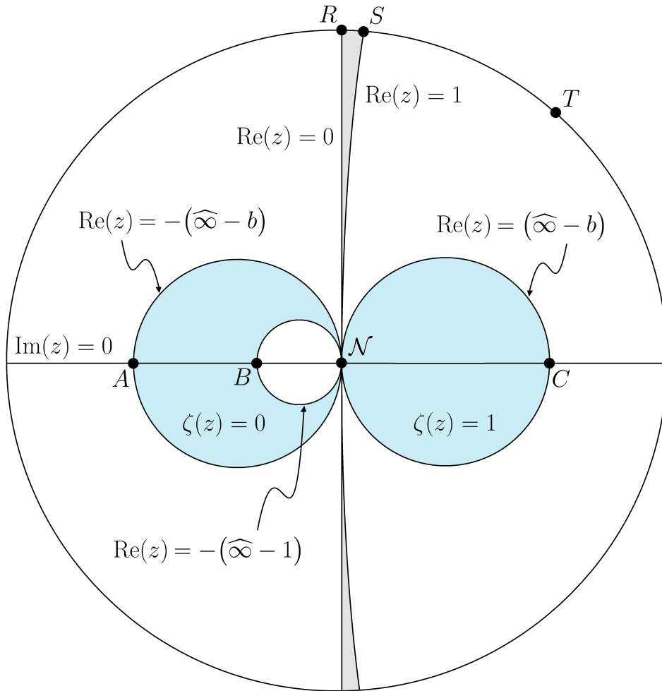
Figure 1: This figure shows a portion of hal_{\Sigma}(\mathcal{N}) . The real axis of \mathbb{C} is the line passing through A and C , and the imaginary axis through R and \mathcal{N} . These axes appear as straight lines in this figure because they are great circles of \mathbb{S}^2 . The circle passing through S and \mathcal{N} (which does not lie entirely within hal_{\Sigma}(\mathcal{N}) ) is the planar line Re(z) = 1 . The critical strip is shaded in gray (not to scale.) The circle passing through A and \mathcal{N} is the planar line Re(z) = -(\infty - b) for some b \in \mathbb{R}_0 > 1 . The circle passing through B and \mathcal{N} is the planar line Re(z) = -(\infty - 1) and we have shown in Reference [18] that \zeta = 0 everywhere in the region between the circles A\mathcal{N} and B\mathcal{N} . The circle passing through \mathcal{N} and C is the planar line Re(z) = (\infty - b) . We have shown in Reference [18] that \zeta = 1 everywhere inside this circle. Note very well: although the circle RST is infinitesimal in radius, everything other than the point \mathcal{N} belongs to \Sigma because we have stated in Definition 1.11 that \Sigma = \mathbb{S}^2 \setminus \mathcal{N} .
